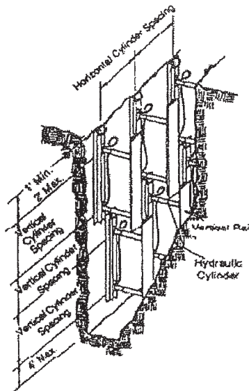
FIG. 3 STACKED
