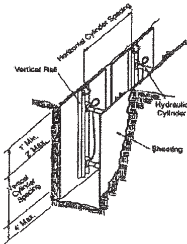
FIG. 1 WITH SHEETING
