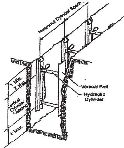
FIG. 2 WITHOUT SHEETING
